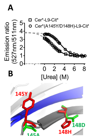
Figure 3. The Cerulean–Citrine intramolecular interface is weaker, due to surface mutations on Cerulean. (A) Fluorescence emission ratio monitored as a function of urea concentration for Cer*-L9-Cit* and Cer*(A145Y/D148H)-L9-Cit*. Curves were fit to a Boltzmann distribution, assuming a transition between closed and opened state. Urea titrations were carried out using 1.5 \mu M protein, in 50 mM Tris-HCl (pH 8), 100 mM NaCl, 10% (v/v) glycerol, at 20 °C. (B) Detail from an alignment of crystal structures for Cerulean (green; 2WSO) and ECFP (red; 2WSN) showing that residue positions 145 and 148 are in close proximity to strand 10 (colored blue), mutations which are known to be crucial in either forming (Q204F, S208F) or disrupting (A206K) a stable dimeric interface. In ECFP, the hydrophobic side group of 145Y (red) clearly points out toward the hydrophobic interface, but in Cerulean the corresponding 145A (green) is buried in the beta-barrel. Also, in ECFP, 148H (red) is oriented parallel to the protein surface, while in Cerulean, 148D (green) points out into the solvent. For clarity, the alternative “B” position of residue 145 is not shown.
