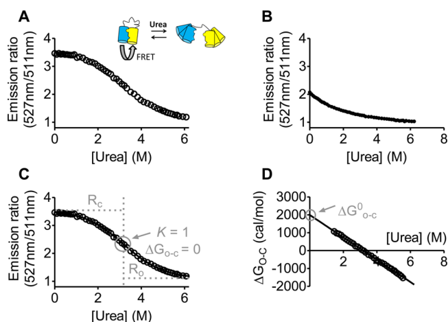
Figure 2. Use of urea titrations to establish the stability of the intramolecular dimer interface in ECFP*-L9-EYFP*. Fluorescence emission ratio of ECFP*-L9-EYFP* (A) or ECFP-L9-EYFP (B) monitored as a function of urea concentration. (C) The data for ECFP*-L9-EYFP* were fit to a Boltzmann distribution, assuming a transition between closed and opened sensor. The emission ratio corresponding to completely closed sensor ( R_c ) and completely opened sensor ( R_o ) are indicated in gray. Also indicated in gray is the titration midpoint ( x_0 ) at which there is an equal amount of closed and opened sensor at equilibrium, so that the equilibrium constant ( K ) is equal to 1 and the Gibbs free energy ( \Delta G_{o-c} ) is equal to 0. (D) Plot showing the linear correlation between the urea concentration and the Gibbs free energy associated with transition from the closed to opened state. Data were fit to a linear model and extrapolated to 0 M urea, providing the standard Gibbs free energy of the complex under native conditions ( \Delta G_{o-c}^0 ), indicated by the gray circle at the intersection of the fit with the Y-axis. Urea titrations were carried out using 1.5 \mu M protein, in 50 mM Tris-HCl (pH 8), 100 mM NaCl, 10% (v/v) glycerol, at 20 °C.
